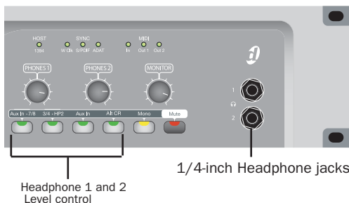
Headphone jacks (Front panel of 003 Rack)
